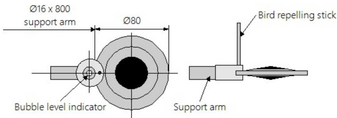
FIGURE 6-1. NR-LITE2 components and dimensions (in millimetres)
